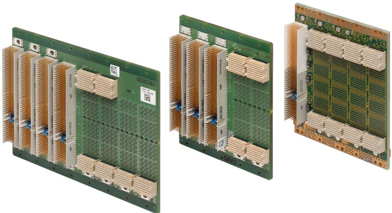
Hybrid Backplanes CPCI & CPCI Serial
